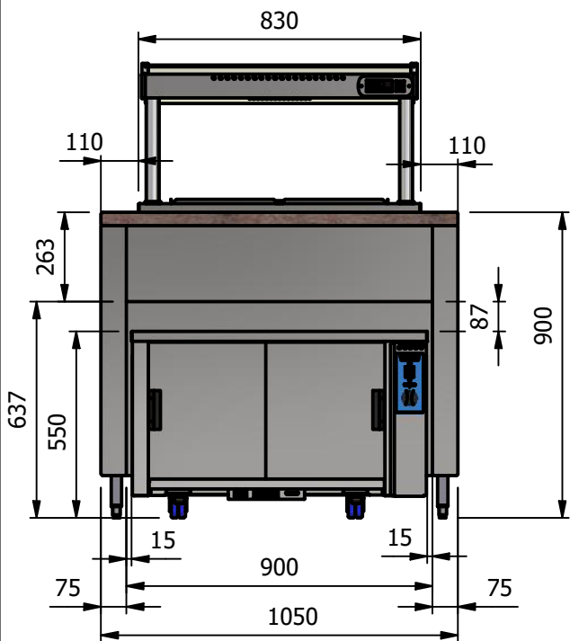
Typical Counter Installation HCRU2 with Size 2 Drop In unit
